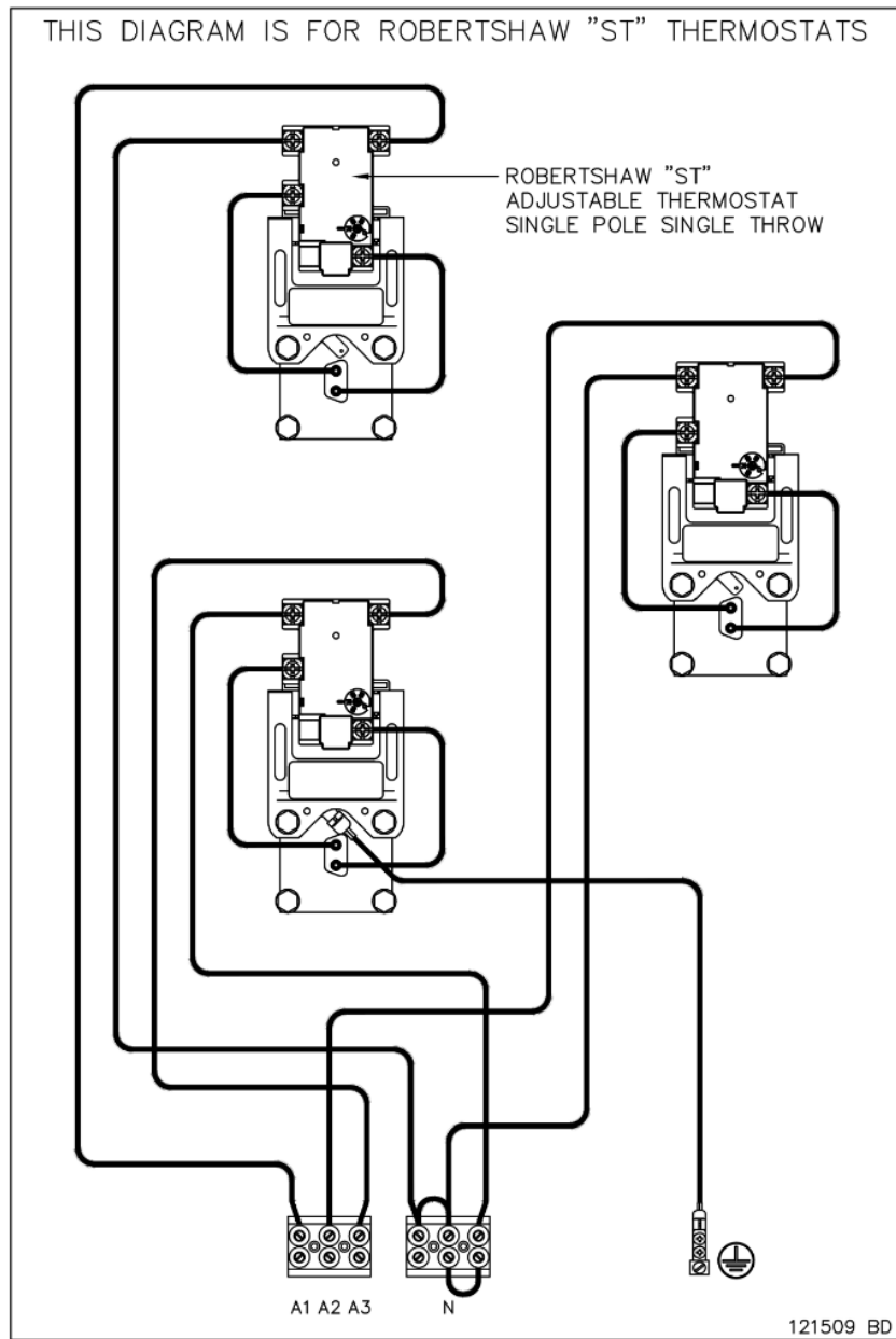
Electrical Circuit for 653 Models – Robertshaw "ST" Thermostats
