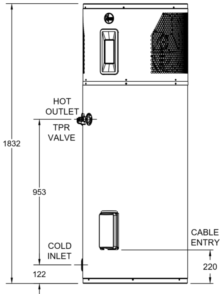
DIMENSIONS AMBIPOWER 280 (551E280) HEAT PUMP WATER HEATER
