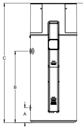
HEAT PUMP 200
